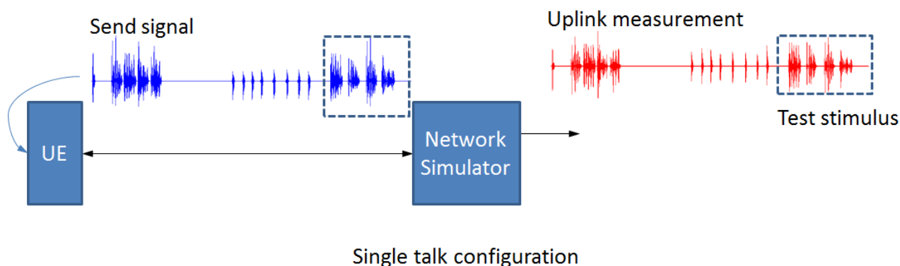
Figure 3a: Signal paths for single talk configuration
