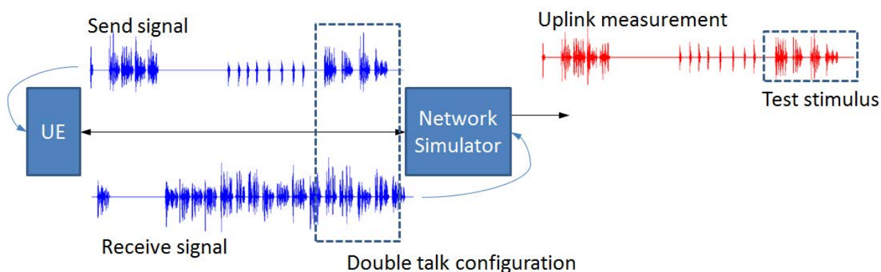
Figure 3b: Signal paths for double talk configuration
