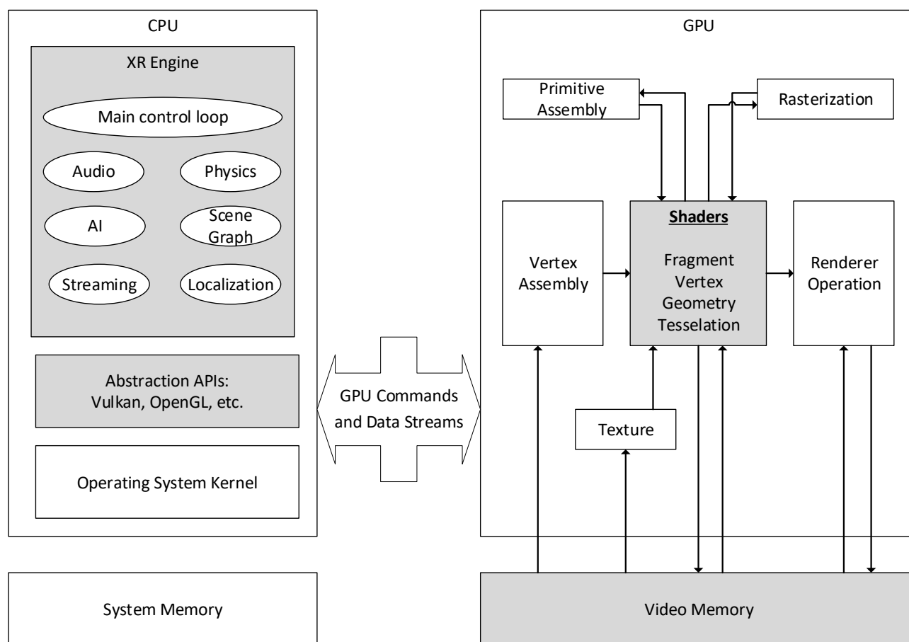
Figure 4.4.1-2: CPU and GPU operations for XR applications
