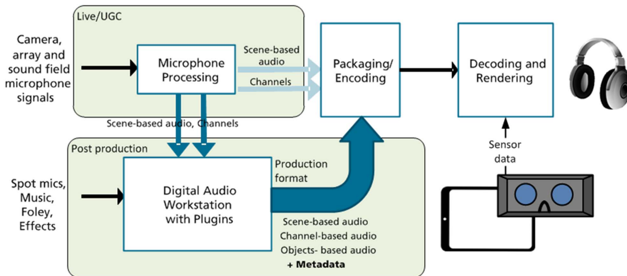
Figure 4.18: Event Multicast to VR enable user equipment
