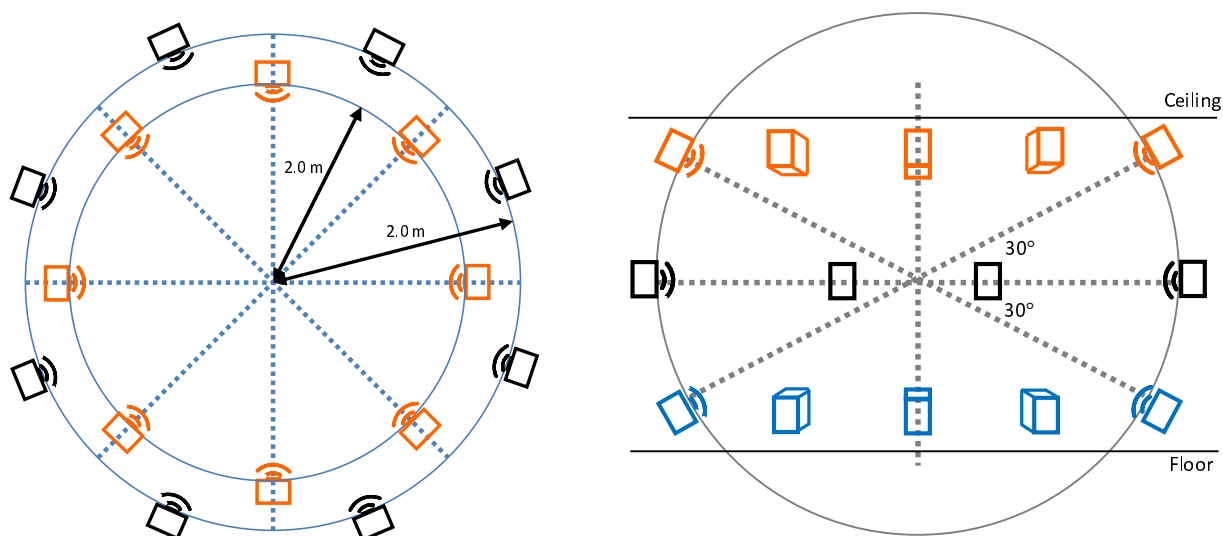
Figure 6.13: 24-loudspeaker setup. The blue speakers are placed at an elevation of -30^\circ degrees, the black speakers at an elevation of 0^\circ degrees and the orange speakers at an elevation of 30^\circ degrees. All speakers are placed at a distance of 2.0 m from the center.
