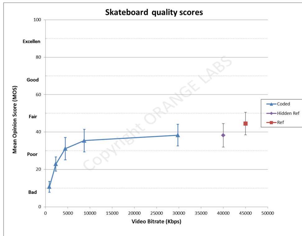
Figure 7.18: Compression quality scores for Skateboard sequence
