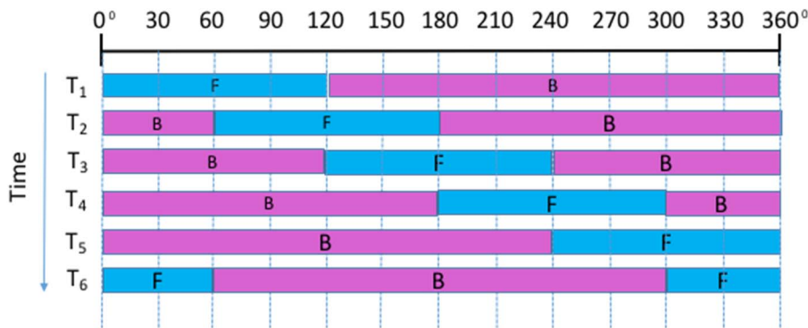
Figure 7.20: Overlapping tiling scheme (panorama view)
