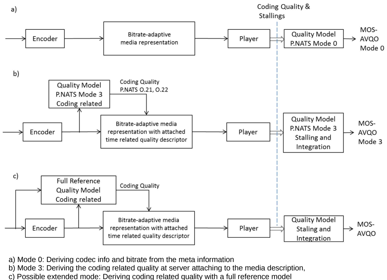
Figure 4.5-1: Possible scenarios for applying the ITU-T P.NATS quality model for monitoring HTTP Adaptive Streaming services
