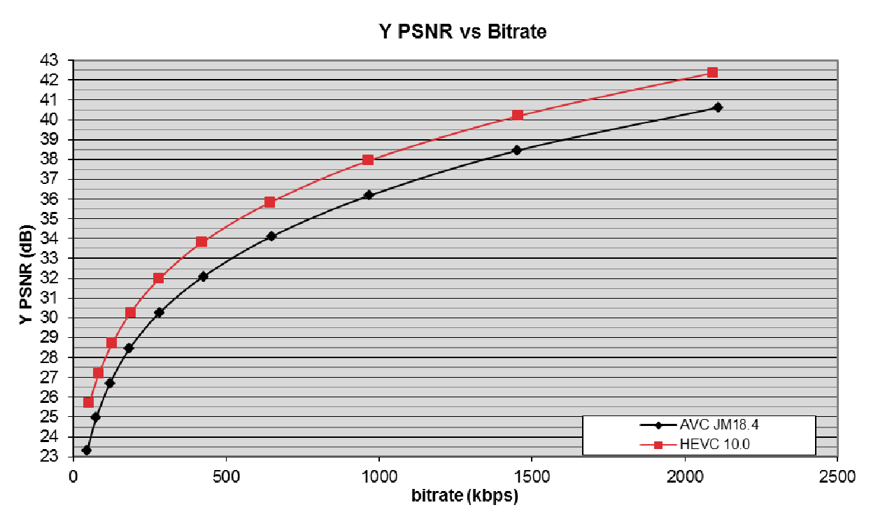
Figure 40: BasketballDrive 240p sequence under closed GOP structure and 2 sec RAP period for MMS test conditions
