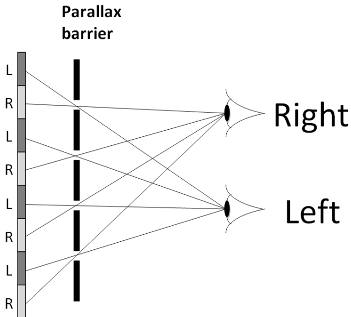
Figure 1: Parallax barrier
