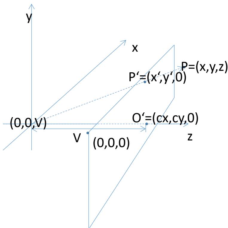
Figure 29: Perspective projection
