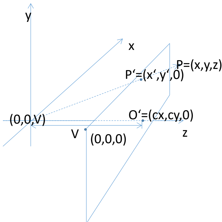
Figure 29: Perspective projection
