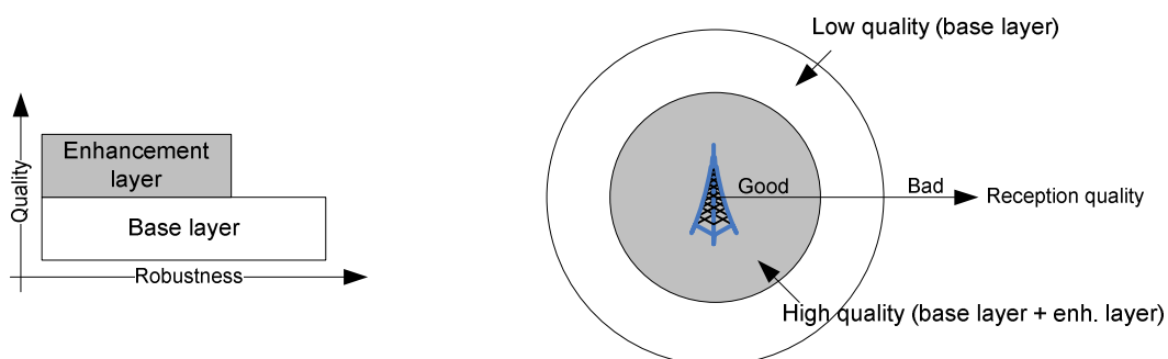
Figure 16: MBMS service with graceful degradation behaviour using unequal error protection with SVC either with temporal, spatial or fidelity scalability or combinations of those
