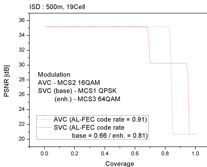
Figure 24: PSNR curves in 19 MBSFN sector layout
