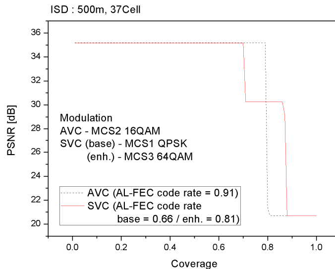
Figure 25: PSNR curves in 37 MBSFN sector layout
