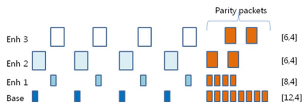
Figure 15: UEP (Unequal Error Protection): Important packets are protected with higher code rate
