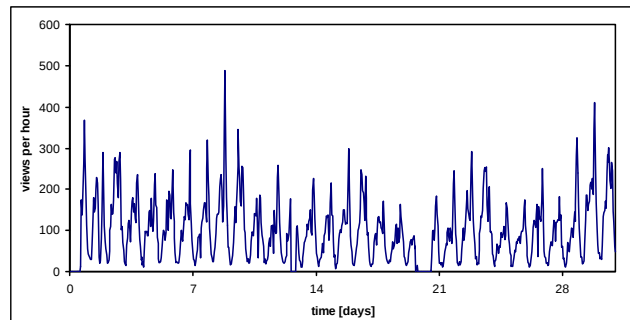
Figure C.1: Requests statistics
