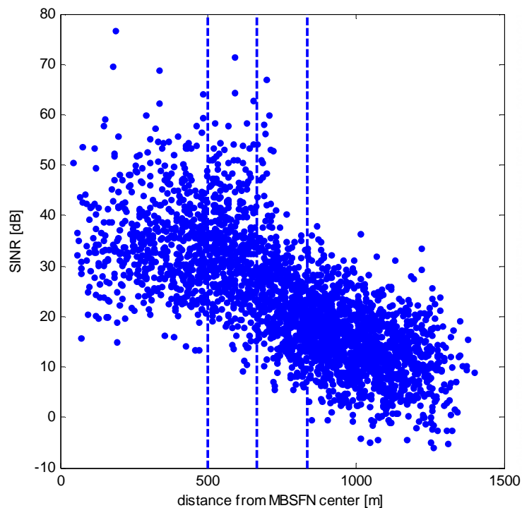
Figure A.9: SINR versus distance from MBSFN center; interfering cells from a second MBSFN
