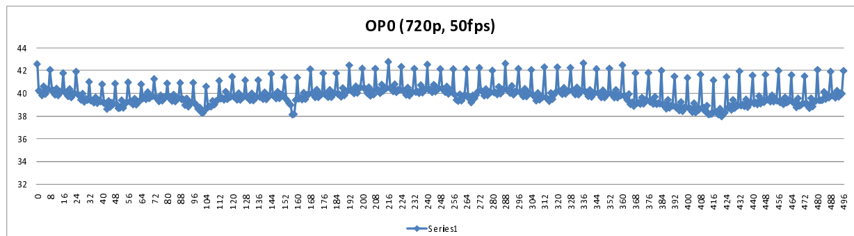
Figure 11: PSNR of each picture for OP0 (IceDance 720p@50fps, GOP 8)
