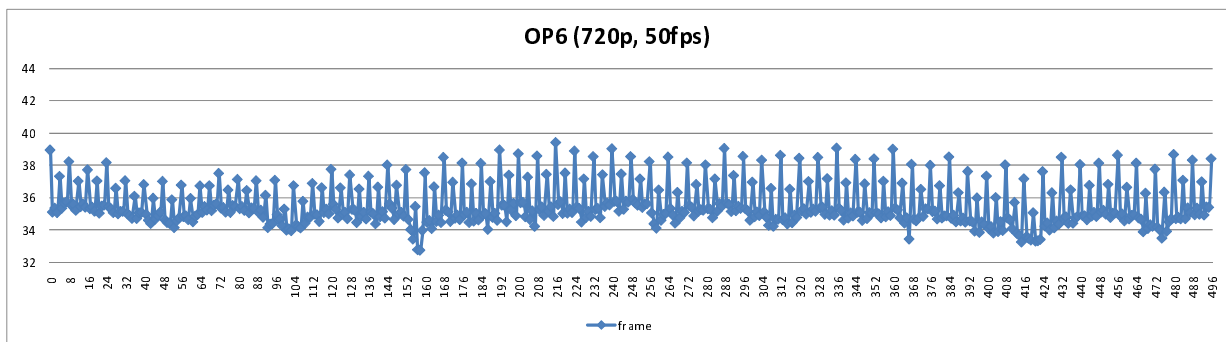
Figure 13: PSNR of each picture for OP6 (IceDance 720p@50fps, GOP 8)
