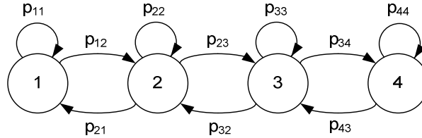
Figure 63: Model for congestion due to cross-traffic
