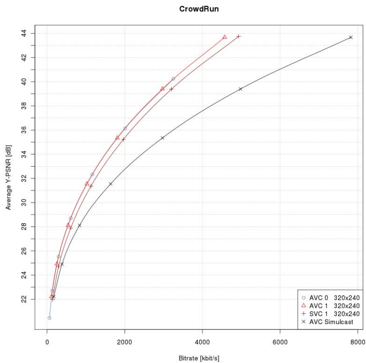
Figure 57: CrowdRun
