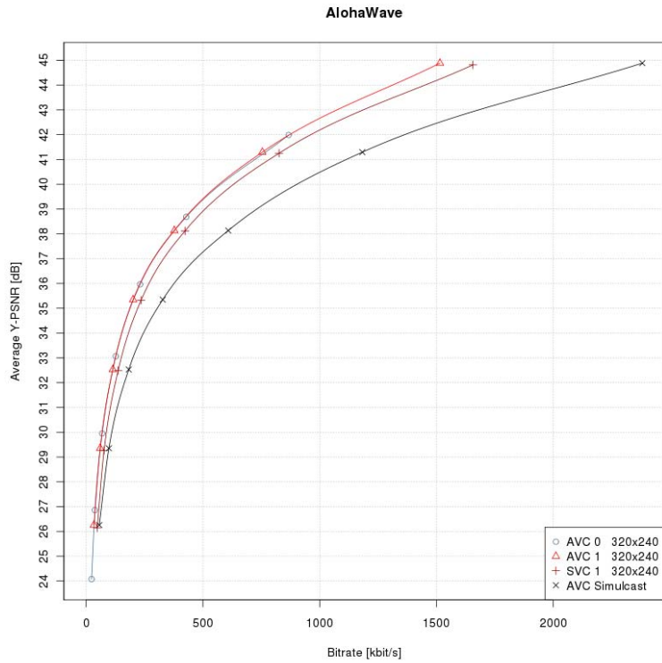
Figure 56: AlohaWave
