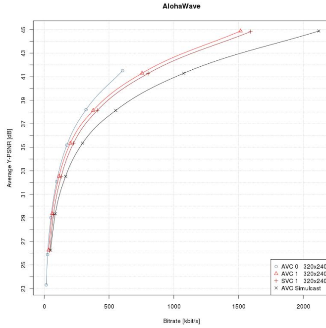
Figure 52: AlohaWave
