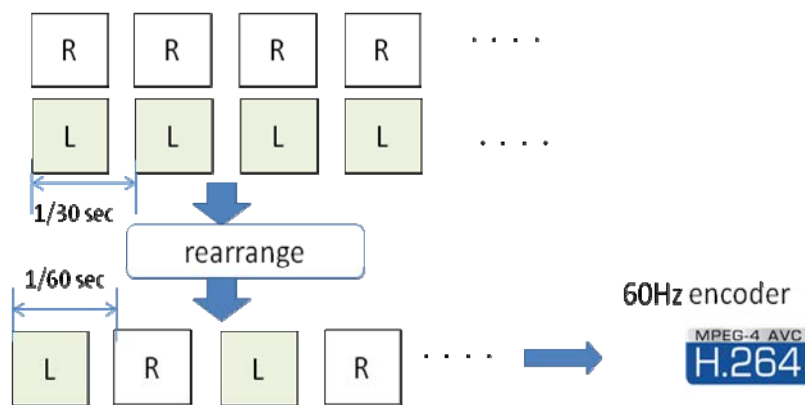
Figure 70: Temporal interleaving
