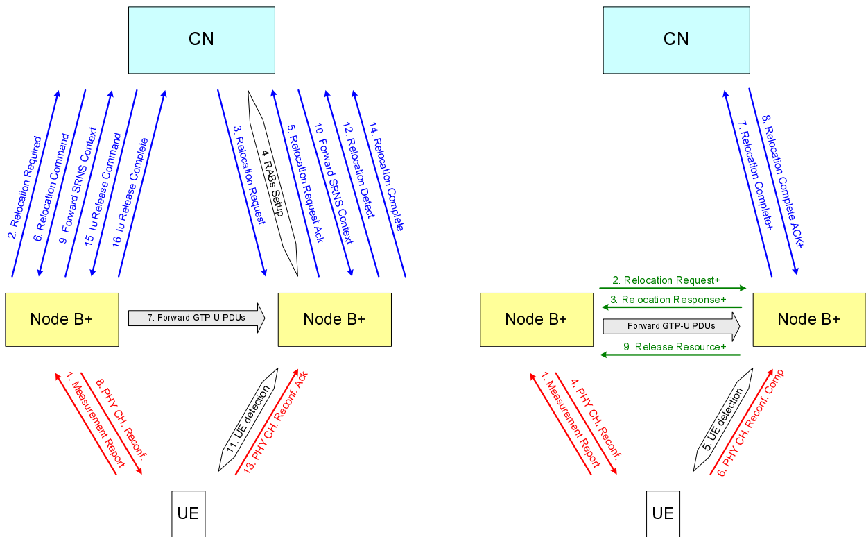
Figure 7.1.7-2: Current vs Enhanced SRNS relocation with hard handover
