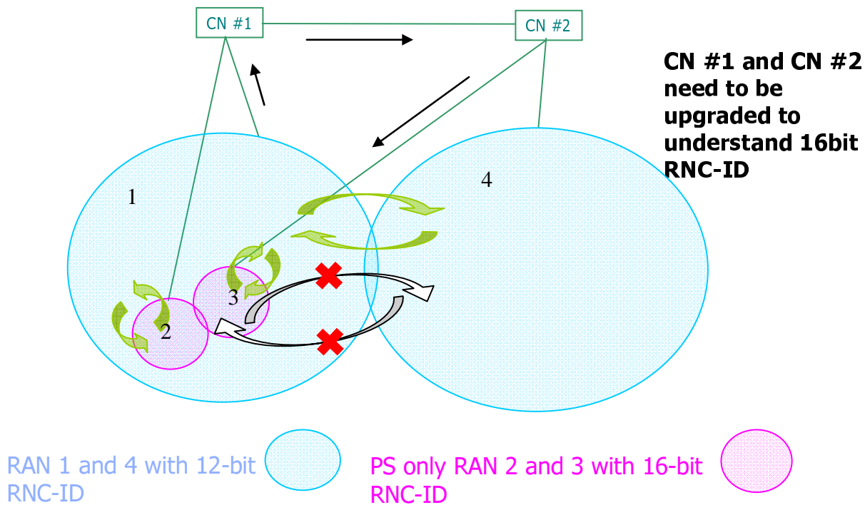
Figure 7.4.3-2: Configuration example for Rule 1 and 2.
