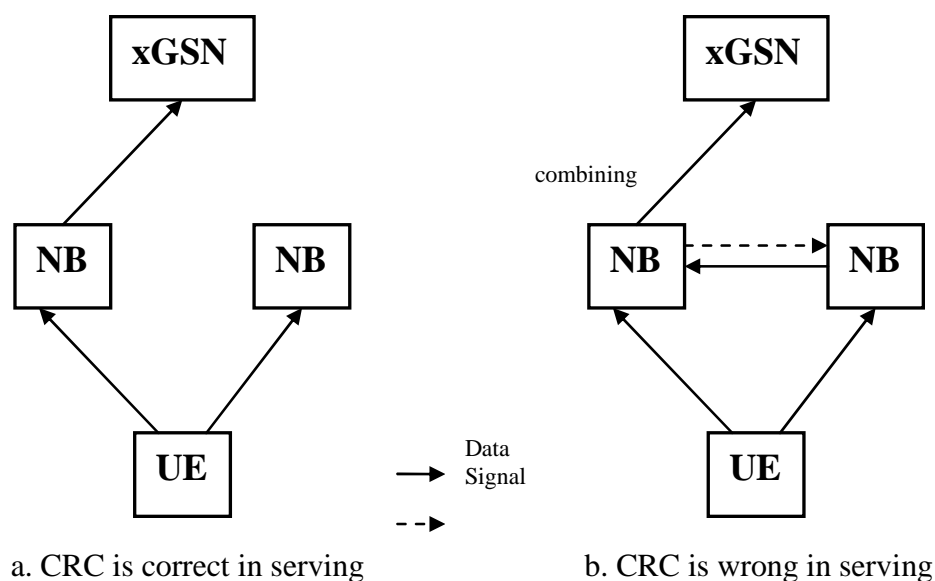
Figure 7.3.1-3: UL MDC in Evolved HSPA Architecture
