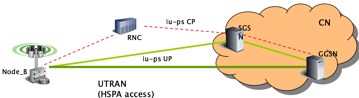
Figure 7.1.3-1: HSPA Evolved Architecture
