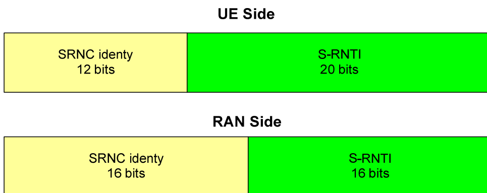
Figure 7.4.1-1: Interpretation of U-RNTI in UE side and RAN side is configured to use the extended RNC ID
