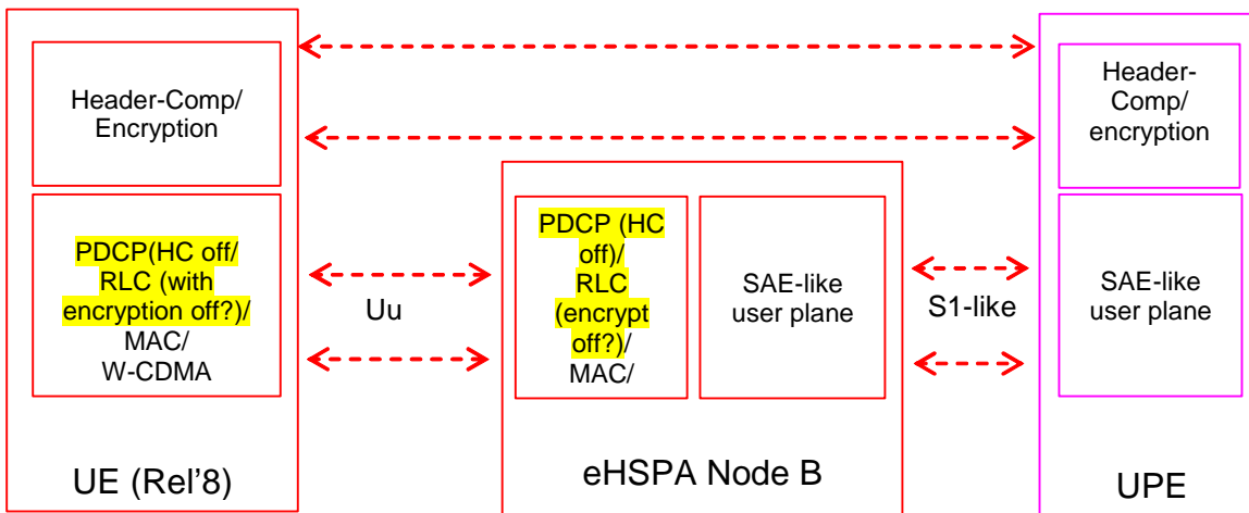
Figure 7.1.5-2: User plane
