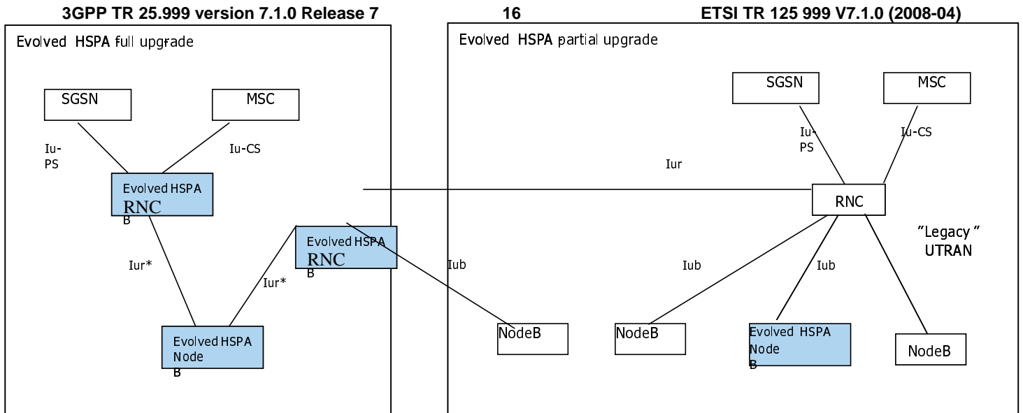
Figure 7.1.2.6-1: Support of Legacy Networks
