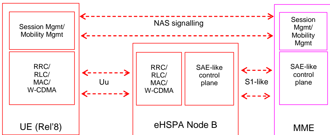
Figure 7.1.5-3: Control plane
