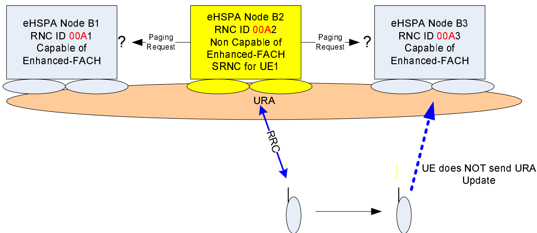
Figure 7.4.3-5 Problematic configuration example (does not follow Rule4)
