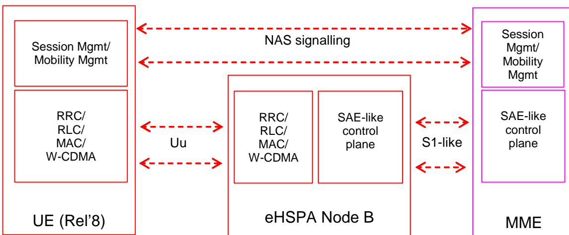
Figure 7.1.5-3: Control plane
