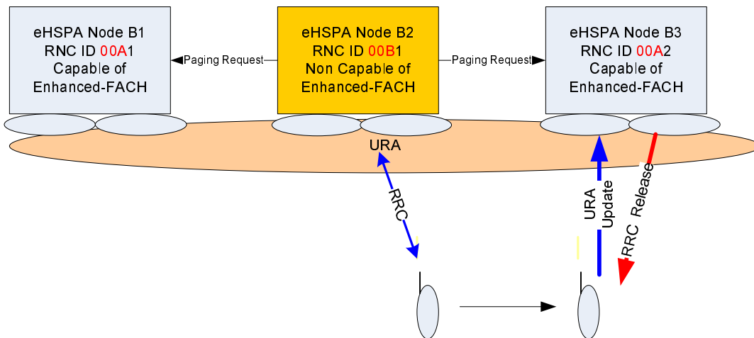
Figure 7.4.3-6 Configuration example for Rule4
