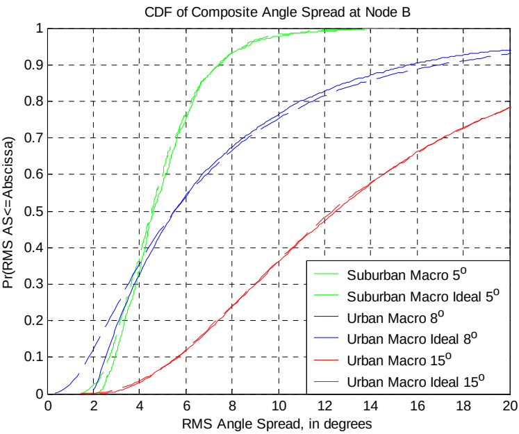
Figure 5.6: BS composite angle spread, simulated versus ideal
