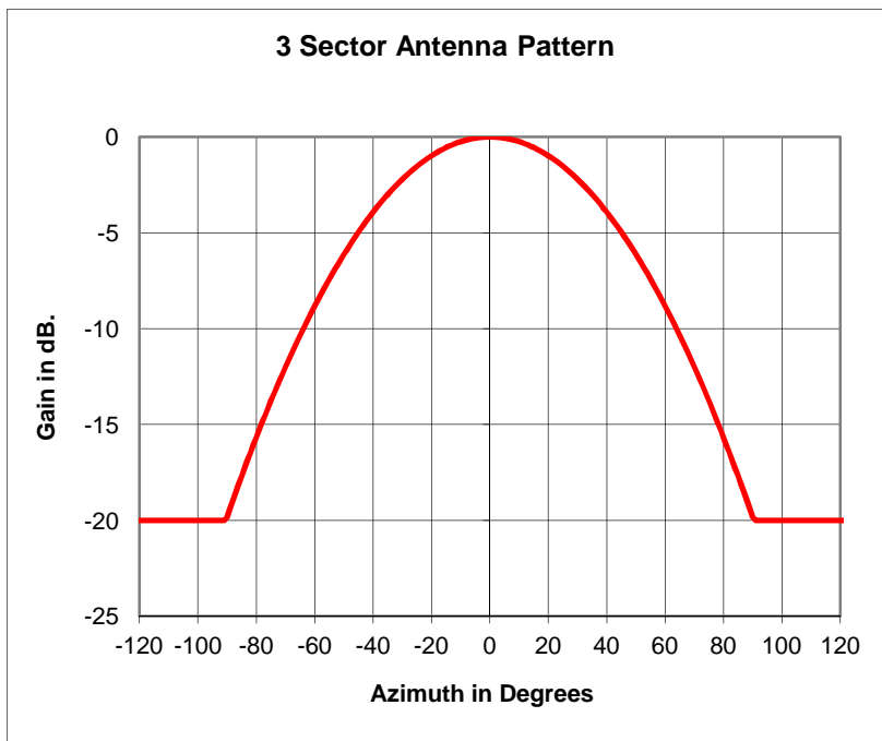
Figure 4.1: Antenna pattern for 3-sector cells
