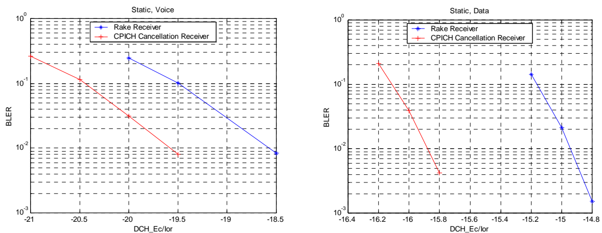
Figure 13: Block error rate as a function of DCH_{Ec/I_{or}} for RAKE and Pilot Mitigation receivers, (using the ideal assumptions of Annex B). Results are shown for Static 12.2 kbps and 64 kbps channels
