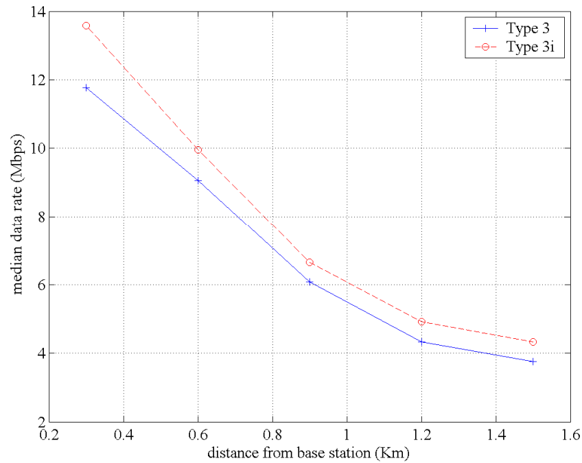
Figure 9.3: Median data rate for users in a highly dispersive channel
