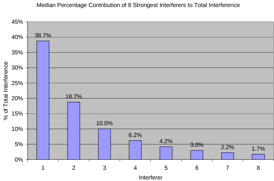
Figure 6.6: 8 Strongest Interferers [10]
