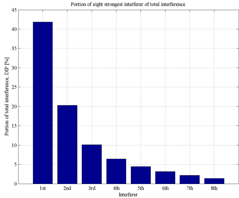
Figure 6.5: 8 Strongest Interferers [9]
