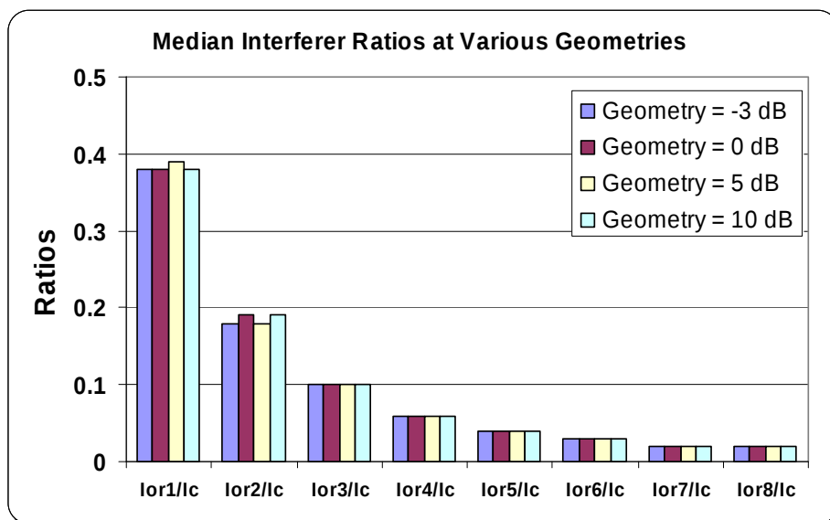
Figure 6.8: 8 Strongest Interferers [12]
