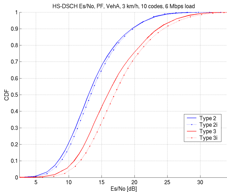
Figure 9.7: HS-DSCH E_s/N_0 distribution of scheduled user
