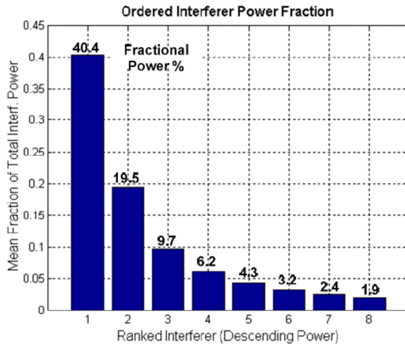
Figure 6.7: 8 Strongest Interferers [11]
