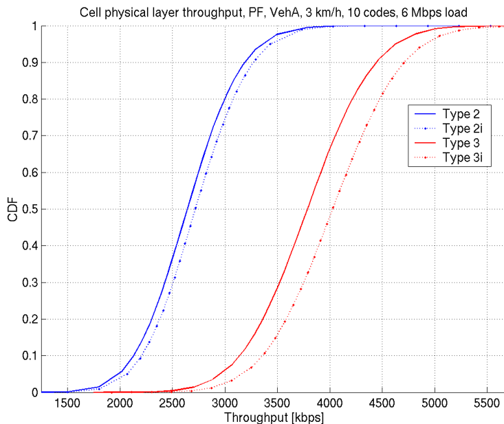
Figure 9.6: Cell throughput
