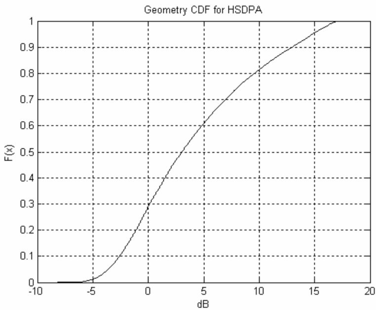
Figure 6.2: Geometry CDF [11]
