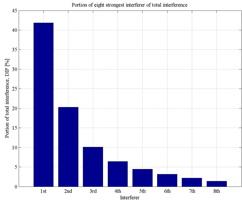
Figure 6.5: 8 Strongest Interferers [9]
