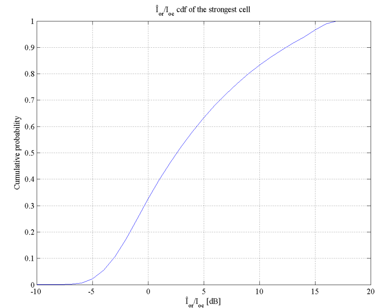
Figure 6.1: Geometry CDF [10]
