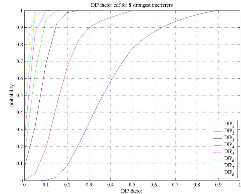
Figure 6.9: Unconditional DIP CDFs [10]
