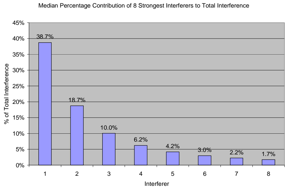
Figure 6.6: 8 Strongest Interferers [10]
