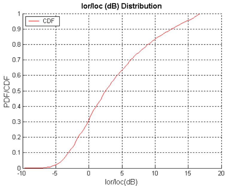
Figure 6.3: Geometry CDF [12]
