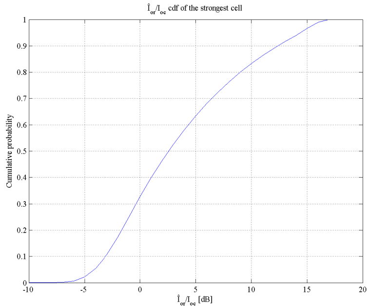
Figure 6.1: Geometry CDF [10]
