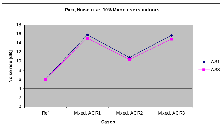
Figure A.14: UL noise rise versus ACIR value with AS1 and AS3
