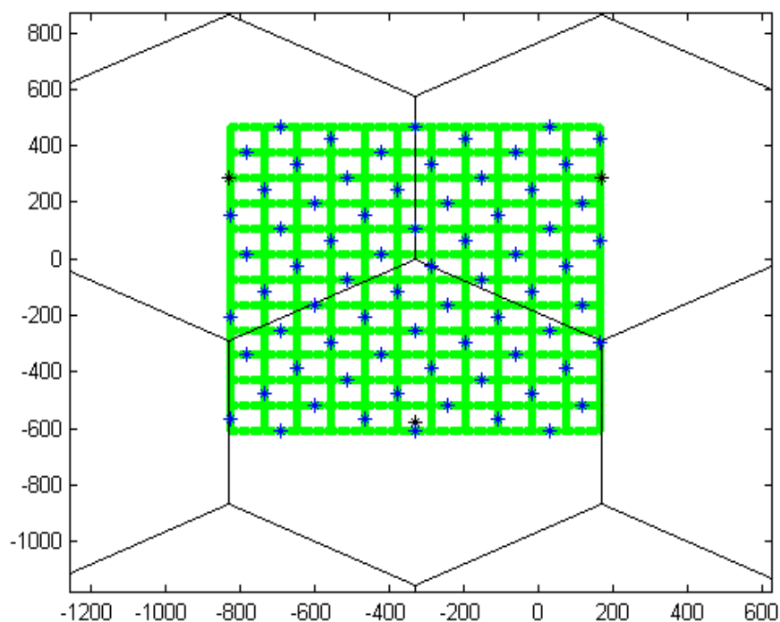
Figure A.1: Macro-Micro network deployment (units are in meter).
