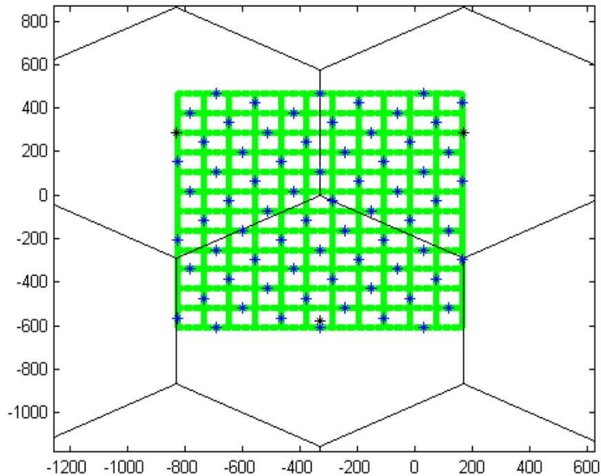
Figure A.6: Macro-Micro network deployment topology, used with 1, 2, 5km macro cell size (zoomed example here for 1 km case).
