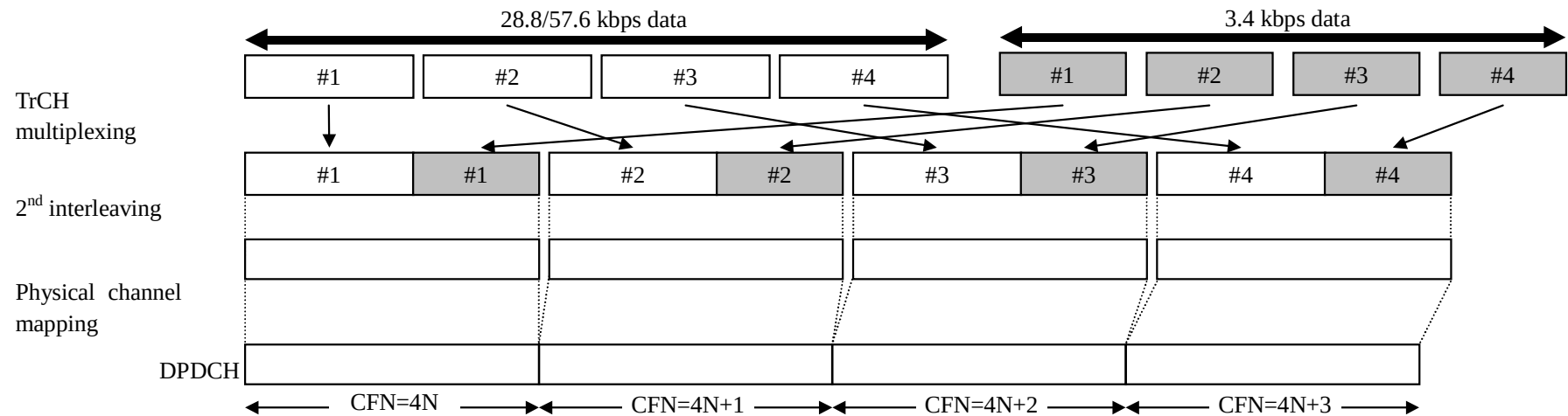
Figure 25: Channel coding and multiplexing example for multiplexing of 28.8/57.6 kbps packet data and 3.4 kbps data
