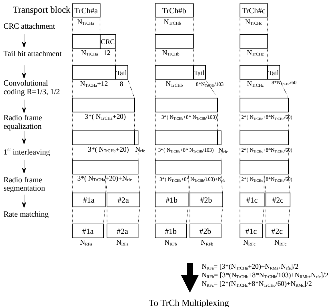
Figure 32: Channel coding and multiplexing example for 12.2 kbps data
