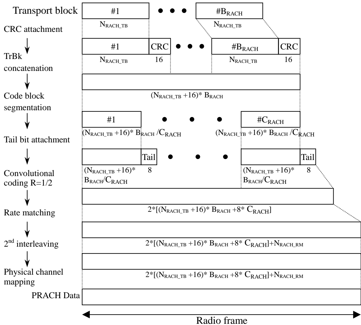
Figure 11: Channel coding and multiplexing example for PRACH
