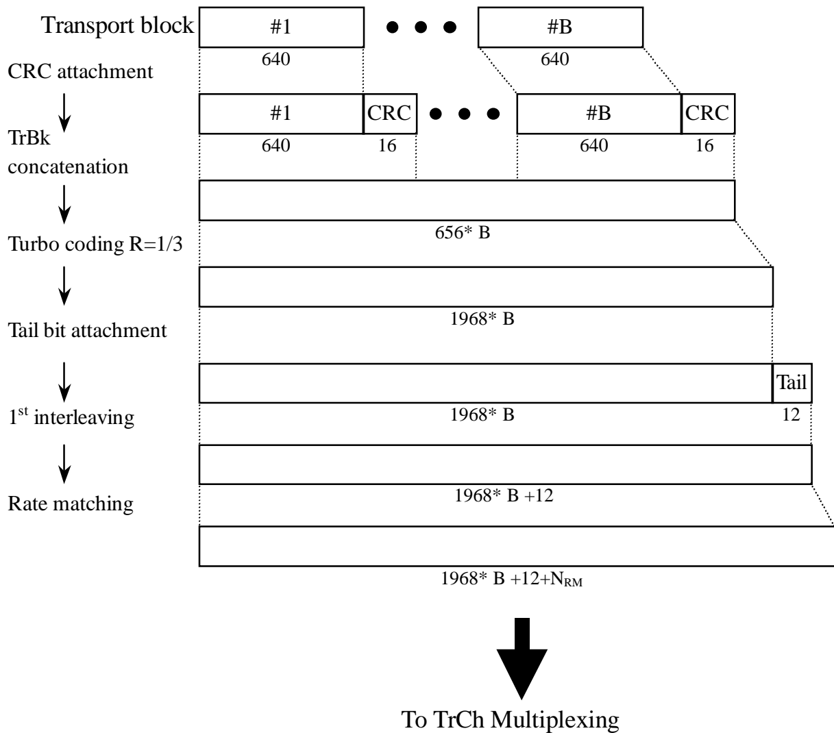
Figure 14: Channel coding and multiplexing example for 64/128/384 kbps packet data
