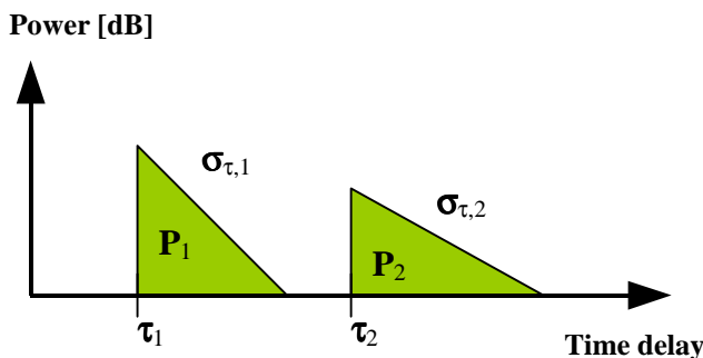
Figure A.1: Channel shape (power delay profile) with multiple clusters.
