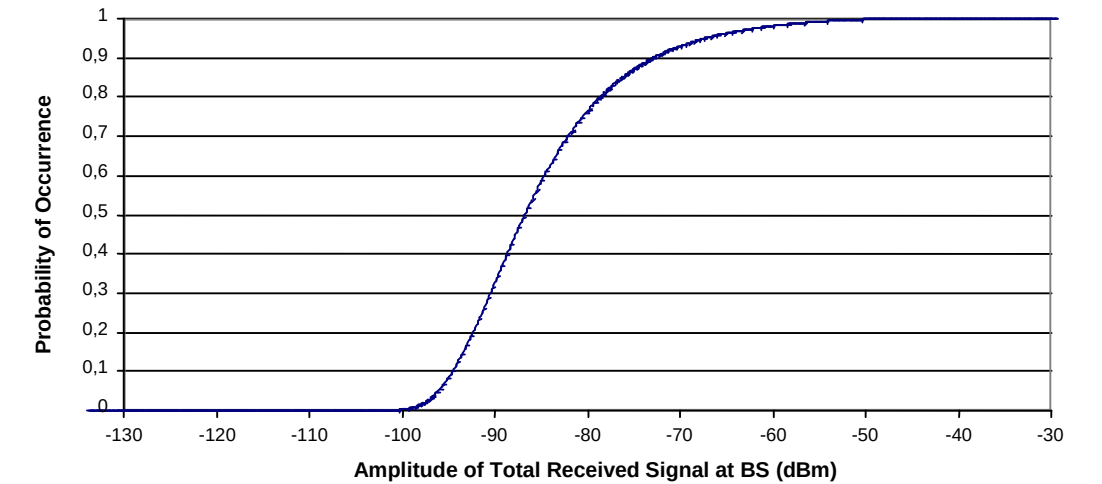
Figure 8.9: CDF of Total Signal for Speech Only System with 5 km Cells and Worst Case Geographic Offset
