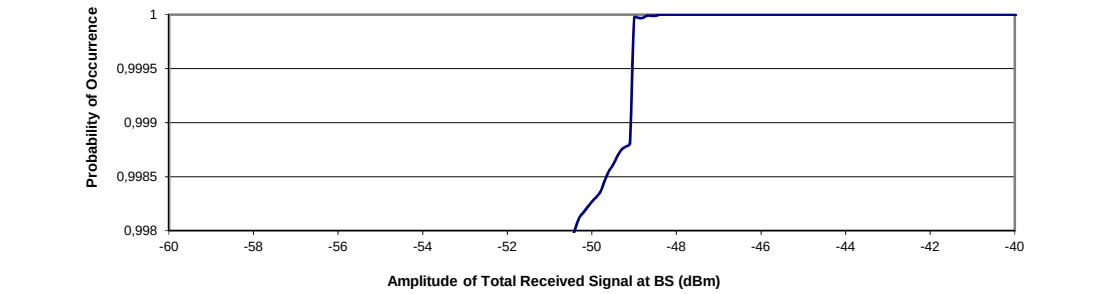
Figure 8.10: CDF of Total Signal for Speech Only System with 5 km Cells and Worst Case Geographic Offset
