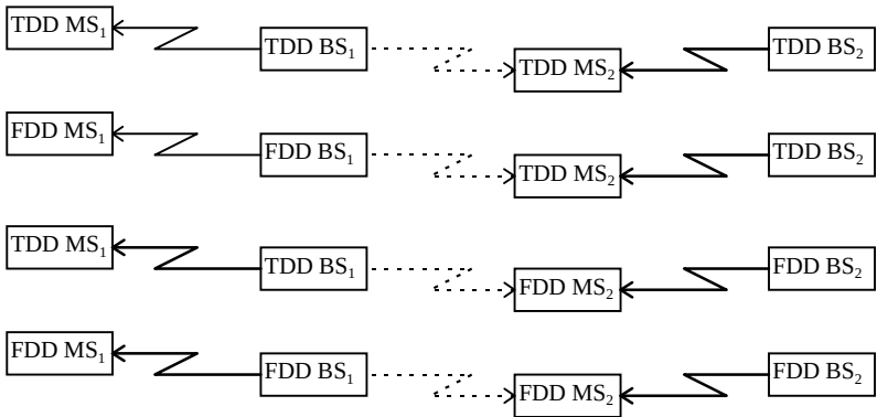
Figure 4.4: Possible BS to MS scenarios
