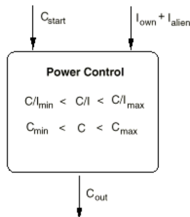
Figure 6.1: C/I based Power Control algorithm
