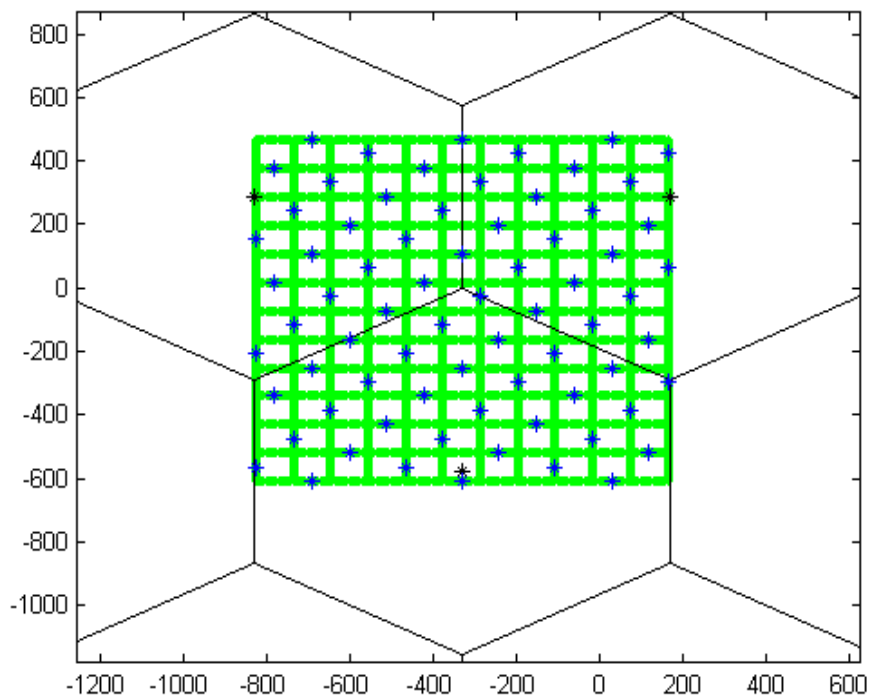
Figure 5.2: Macro-Micro network deployment topology (zoomed example for 1km interfering macro cell size)
