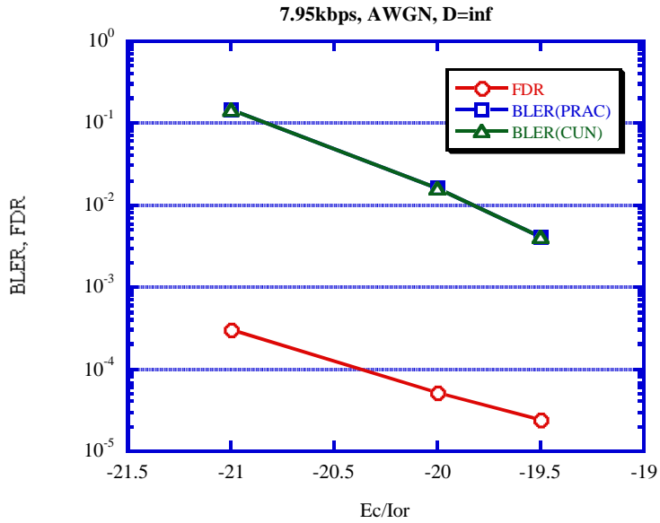
Figure 15.2: Ec/Ior vs. BLER (STATIC, 7,95 k)
