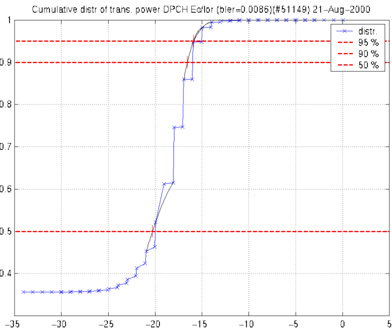
Figure 56: Cumulative distribution of transmission power DPCH_Ec/Ior when compressed mode is on. TGL = 4 slots
