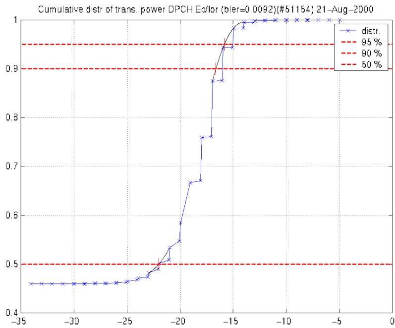
Figure 60: Cumulative distribution of transmission power DPCH_Ec/Ior when compressed mode is on. TGL = 14 slots
