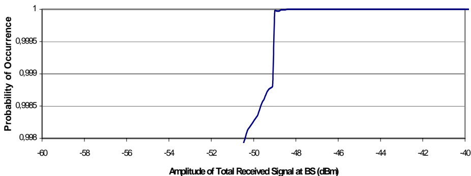
Figure 25: CDF of Total Signal for Speech Only System with 5 km Cells and Worst Case Geographic Offset
