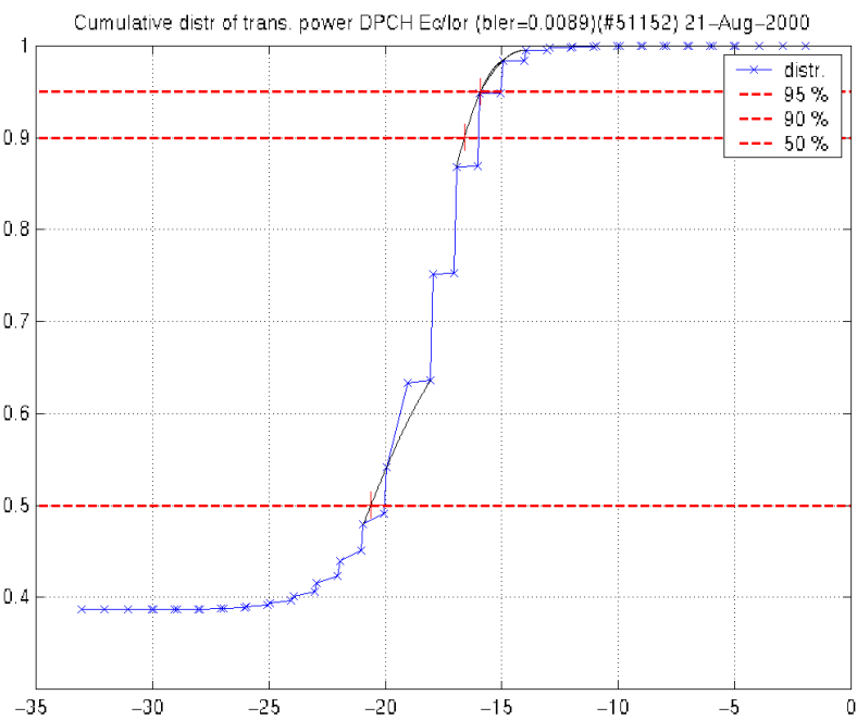
Figure 57: Distribution of transmission power DPCH_Ec/Ior when compressed mode is on. TGL = 7 slots. The gap in the PDF probably exists because of the bin widths
