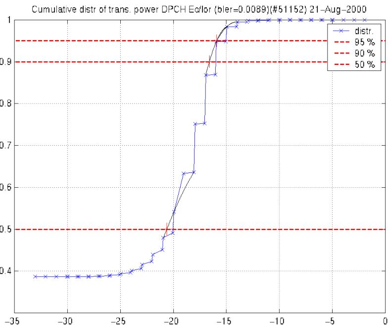
Figure 58: Cumulative distribution of transmission power DPCH_Ec/Ior when compressed mode is on. TGL = 7 slots
