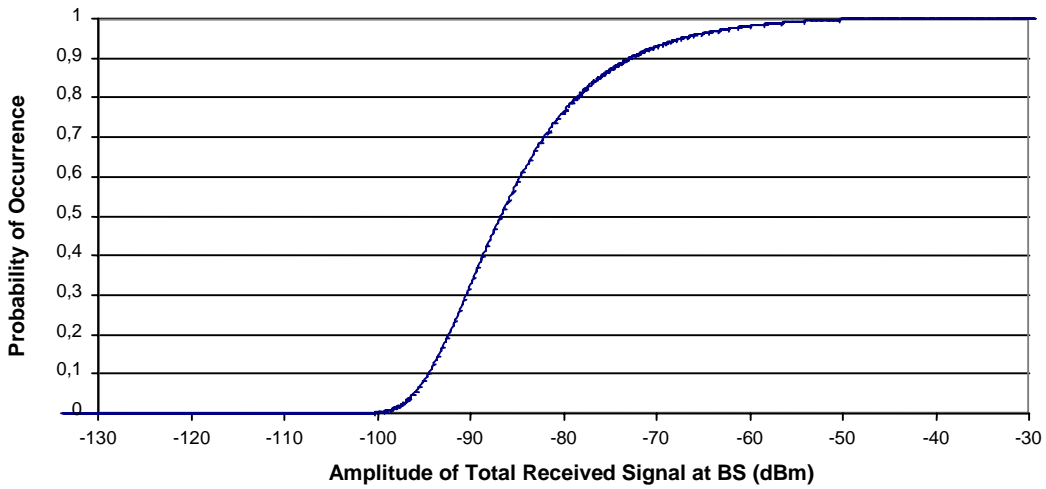
Figure 24: CDF of Total Signal for Speech Only System with 5 km Cells and Worst Case Geographic Offset
