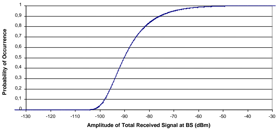
Figure 26: CDF of Total Signal for Mixed Speech and Data System with 5 km Cells and Worst Case Geographic Offset
