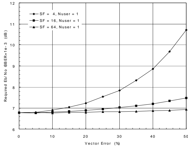
Figure 32: Degradation for the case of single code transmission
