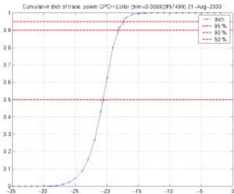
Figure 54: Cumulative distribution of transmission power DPCH_Ec/Ior when compressed mode is off
