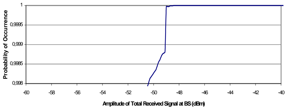
Figure 25: CDF of Total Signal for Speech Only System with 5 km Cells and Worst Case Geographic Offset
