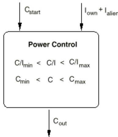
Figure 11: C/I based Power Control algorithm
