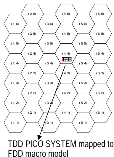
Figure 31D: TDD pico and FDD Macro evaluation layout; pico model chosen from [31]
