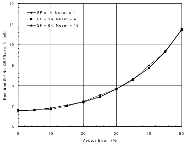
Figure 33: Degradation for the case of a quarter of the maximum traffic load
