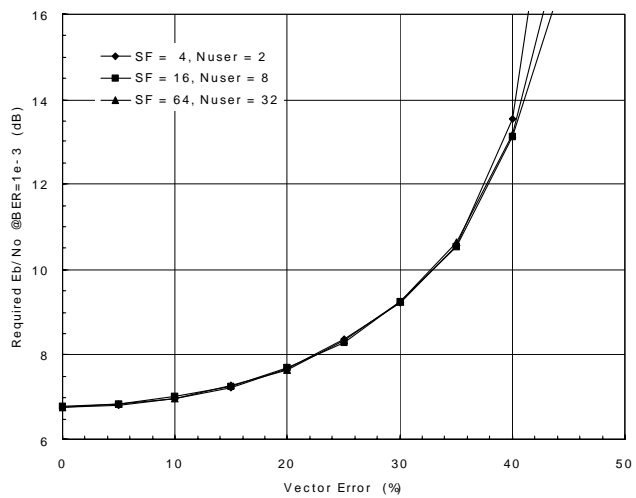
Figure 34: Degradation for the case of a half the maximum traffic load
