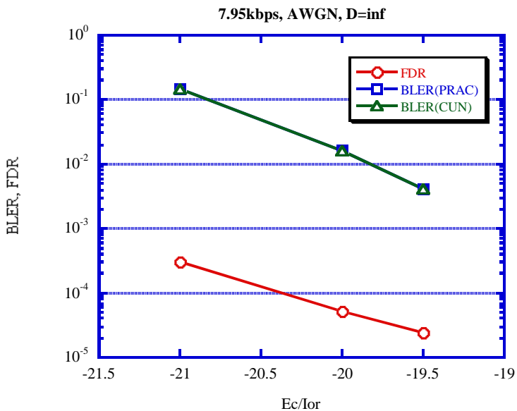
Figure 48: Ec/Ior vs. BLER (STATIC, 7,95 k)
