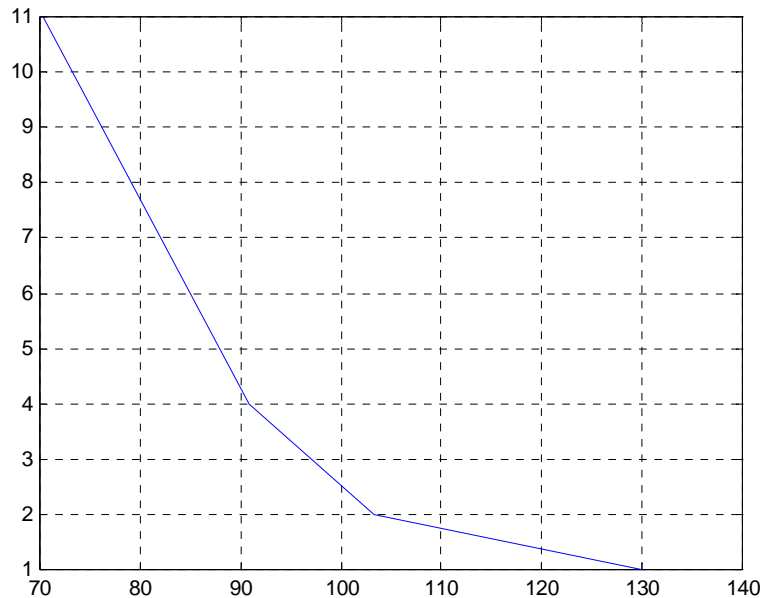
Figure 31A: FDD capacity loss along the coupling loss between FDD macro BS and TDD pico system.
