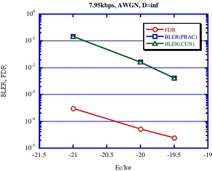
Figure 48: Ec/Ior vs. BLER (STATIC, 7,95 k)
