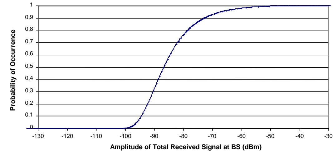
Figure 24: CDF of Total Signal for Speech Only System with 5 km Cells and Worst Case Geographic Offset
