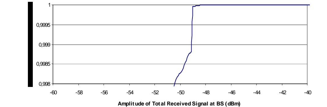
Figure 25: CDF of Total Signal for Speech Only System with 5 km Cells and Worst Case Geographic Offset
