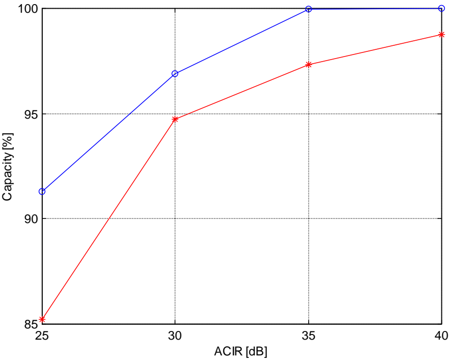
Figure 29: Relationship between ACIR and capacity loss for speech in DL in the intermediate and worst case
