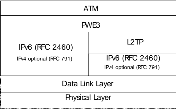
Figure 6-34: Bearer for Control plane (RANAP), Transport Network control plane (ALCAP) and user plane with PWE3 tunneling protocol.
