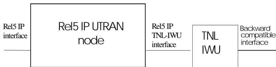
Figure 7-6: A TNL Interworking Unit present between the IP UTRAN Node and the ATM UTRAN Node
