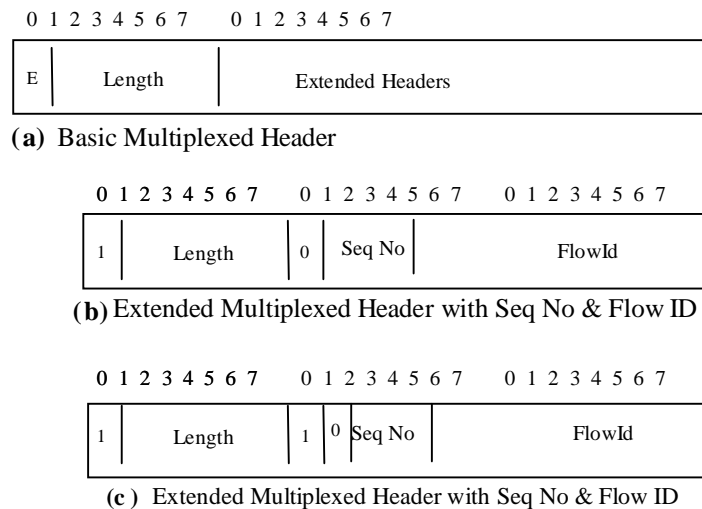
Figure 6-5: Formats of Multiplexed Header
