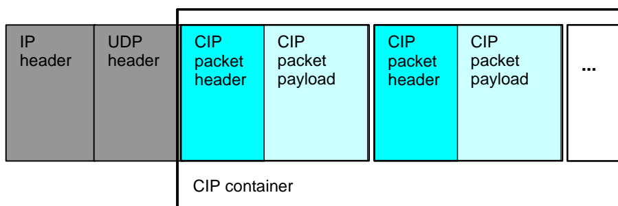
Figure 6-1-1: Generic CIP Container format
