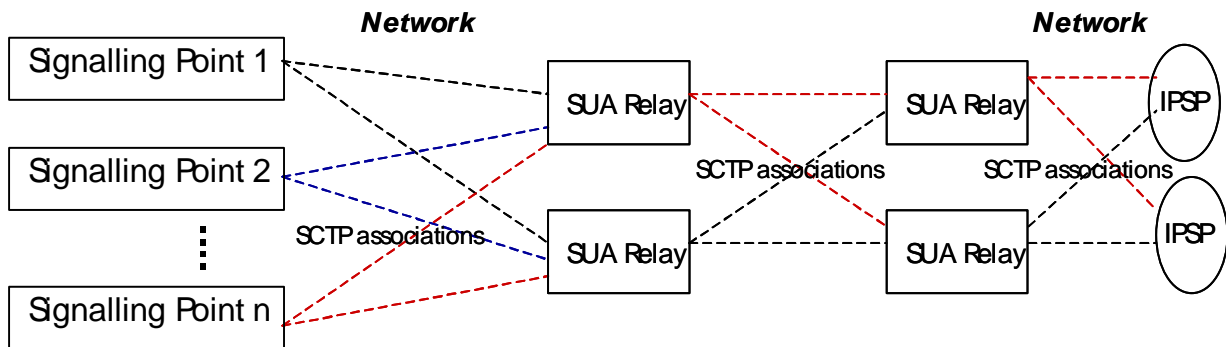
Figure 6-24: Interconnecting Operator Networks with SUA
