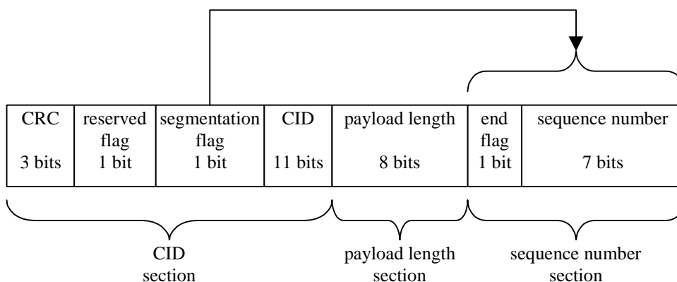
Figure 6-3-3: CIP packet header format
