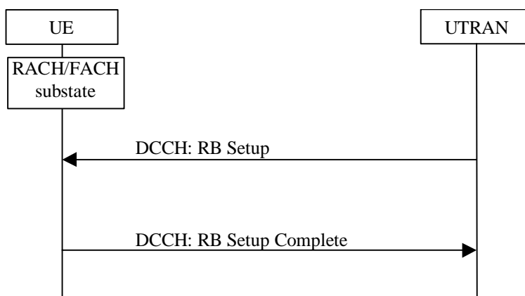
Figure B-1: Radio Bearer setup on common transport channel
