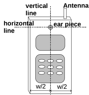
Figure 5.3: Reference lines at a mobile handset (Device Under Test (DUT)). W is the width of the chassis [19].
