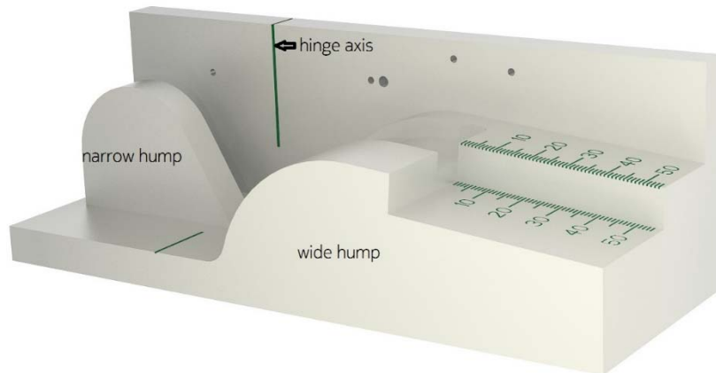
Figure 5.1.6.2-1 Alignment Tool B and right-handed fold hand phantom with a spacer. Use left-handed (mirror-imaged) spacers with left-handed phantoms.
