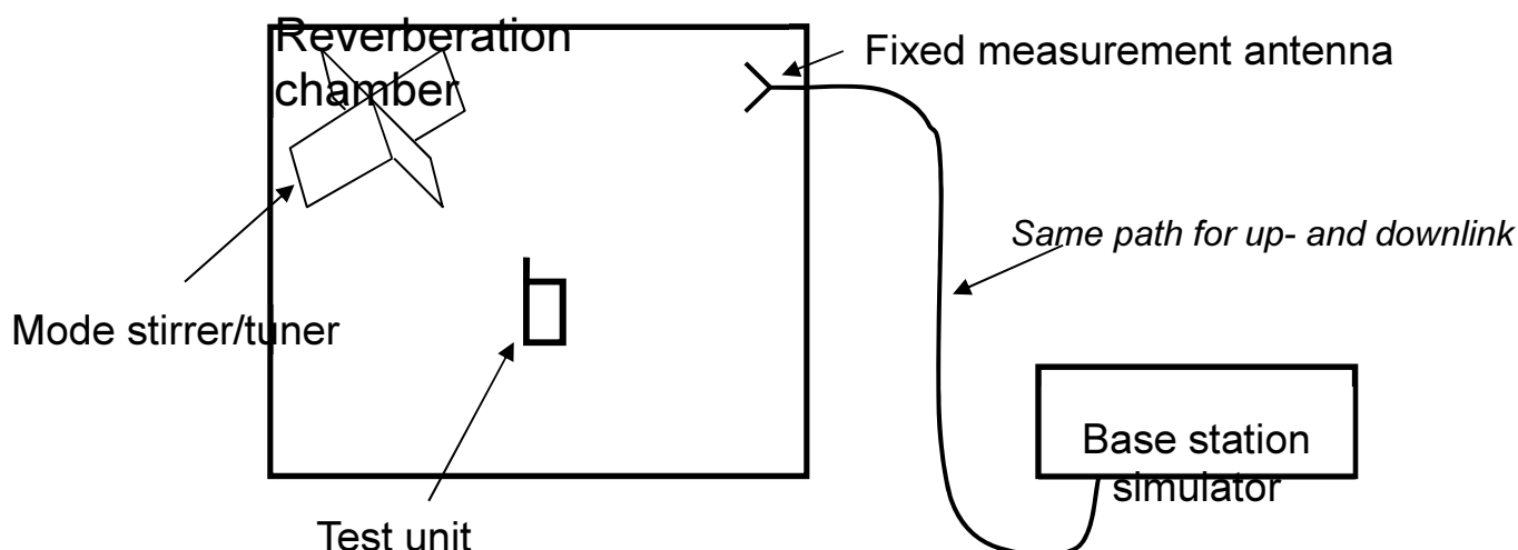
Figure E.1: Schematic picture of the reverberation chamber measurement setup
