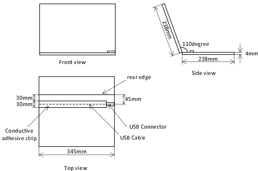
Figure 5.5: The structure and dimension of the laptop ground plane phantom
