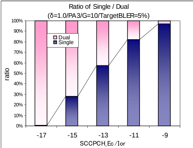
Fig. 5.1.4.1.4 Ratio between 1 and 2 antenna in PA3 ( \delta=1.0 ).
