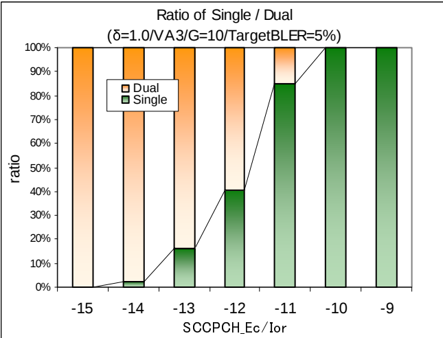
Fig. 5.1.4.1.8 Ratio between 1 and 2 antenna in VA3 ( \delta=1.0 ).
