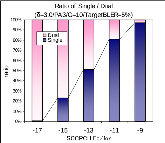
Fig. 5.1.4.1.6 Ratio between 1 and 2 antenna in PA3 ( \delta=3.0 ).
