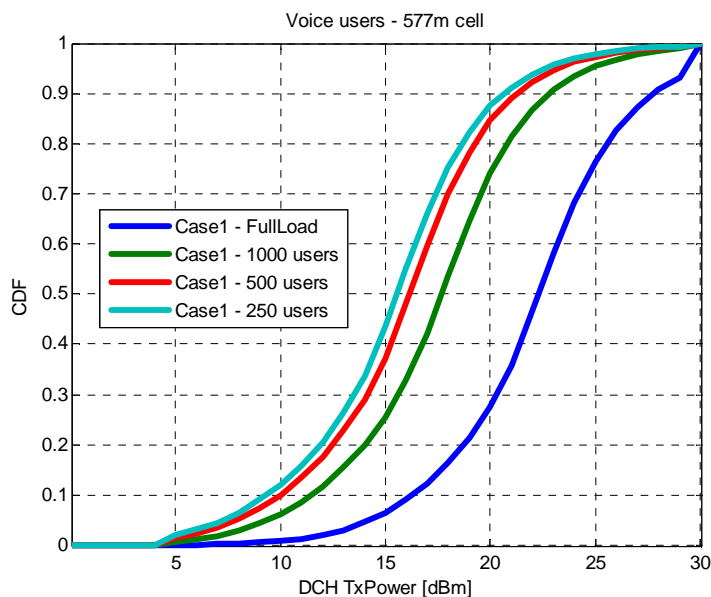
Figure 9: Macro-cell network simulation results showing UE code power CDF
