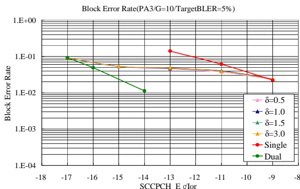
Figure 5.1.4.1.1: BLER performance in PA3.
