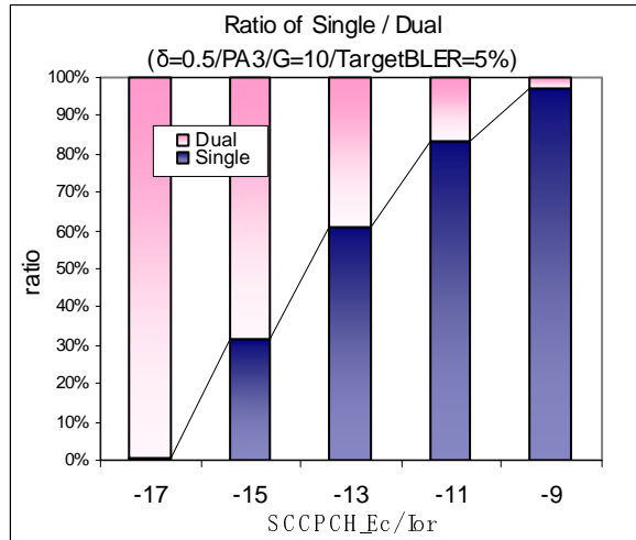
Fig. 5.1.4.1.3 Ratio between 1 and 2 antenna in PA3 ( \delta=0.5 ).
