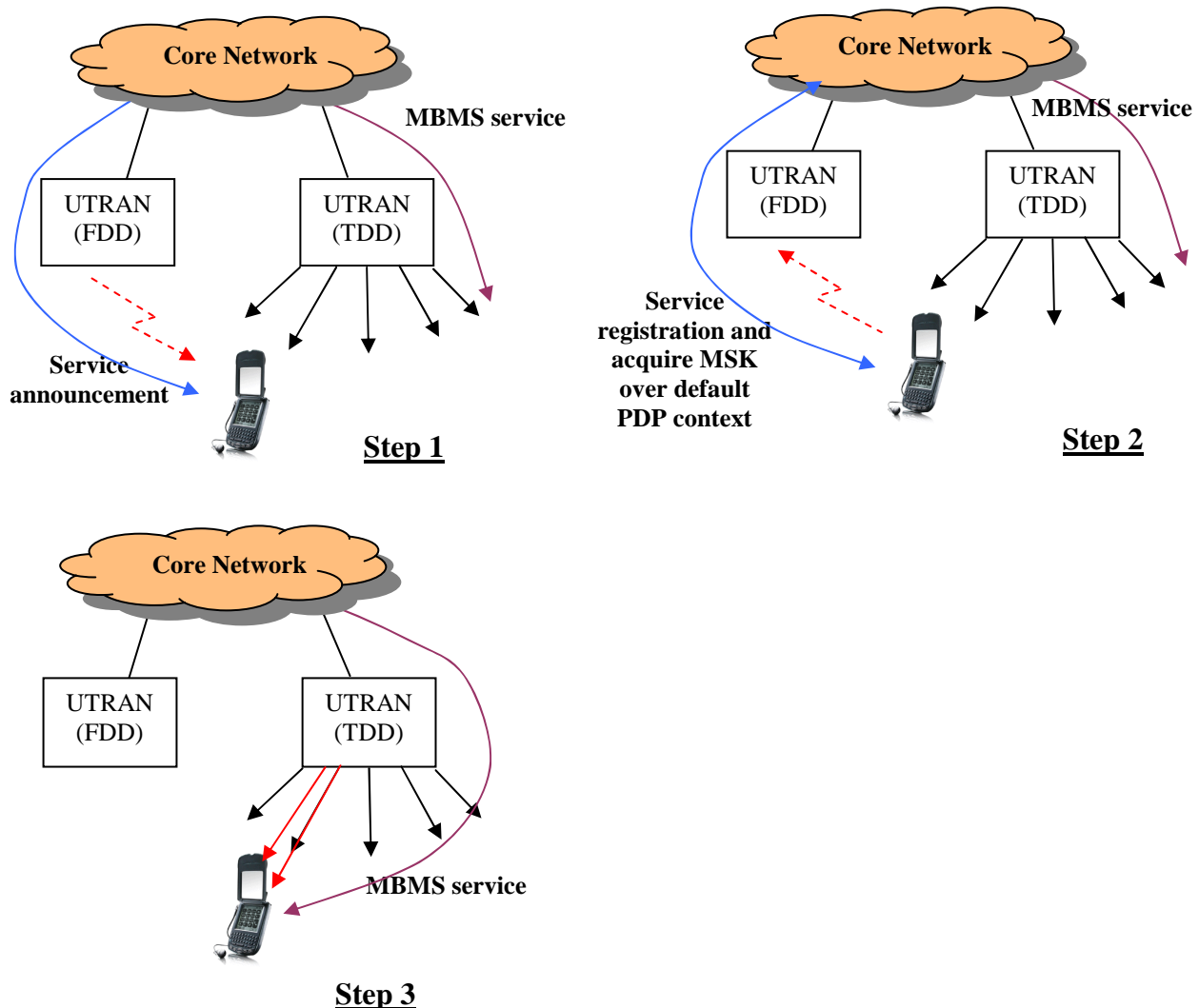
Figure 10: Steps involved in reception of MBMS service over TDD according to non-integrated RAN scenario.
