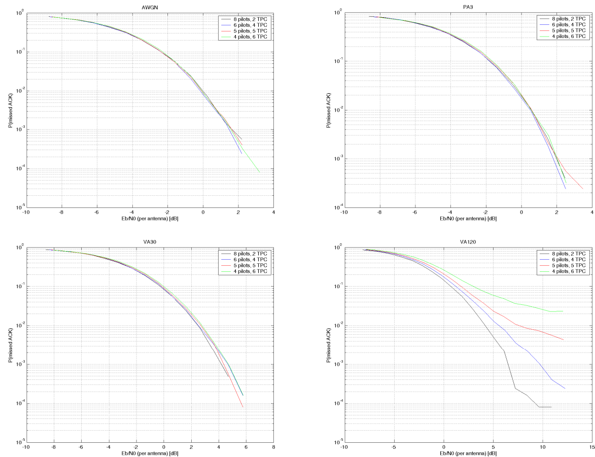
Figure 4.1.2.2.2-6: Probability of missed ACK for different UL DPCCH slot formats and various channel models
