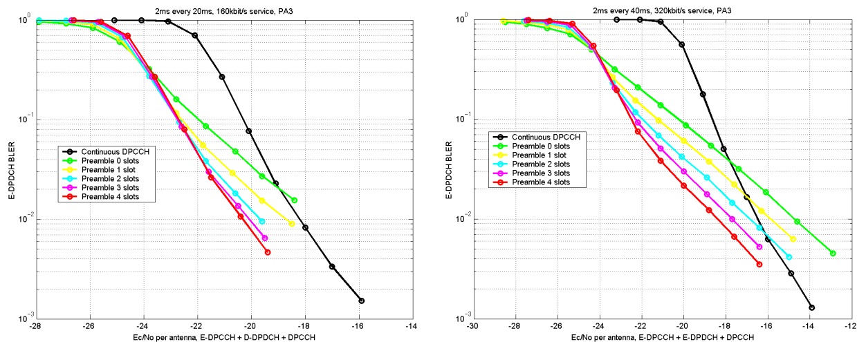
Figure 4.2.2.1-2: BLER vs. E_c/N_0 for different preamble lengths. Pedestrian A, 3 km/h
