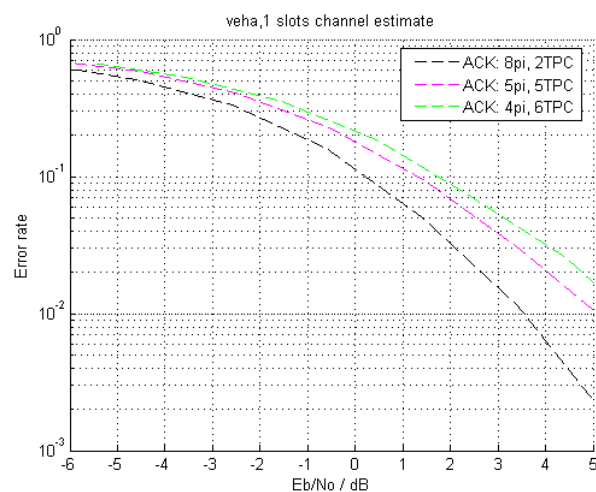
Figure 4.1.2.2-4: ACK performance in VA120, 1 slot channel estimation, with TPC-assistance
