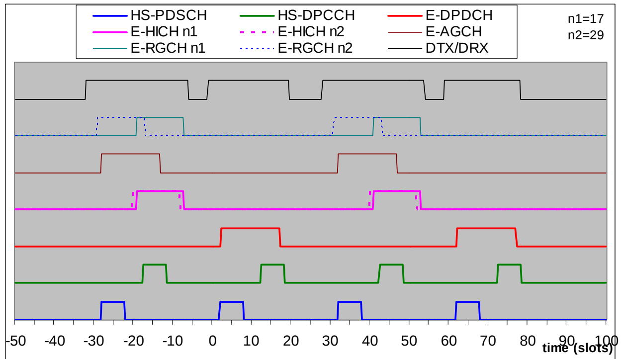
Figure 4.5.2.A.5-1: UE in handover region, 10ms E-DCH, DRX mode 1/4, in soft handover, 23% sleep time
