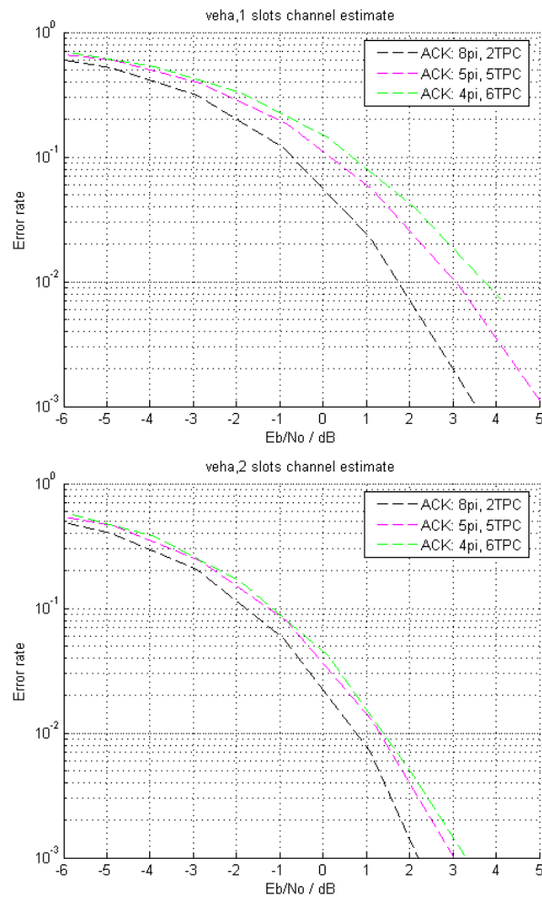
Figure 4.1.2.2-3: ACK performance in VA30, 1 and 2 slot channel estimation, both with TPC-assistance
