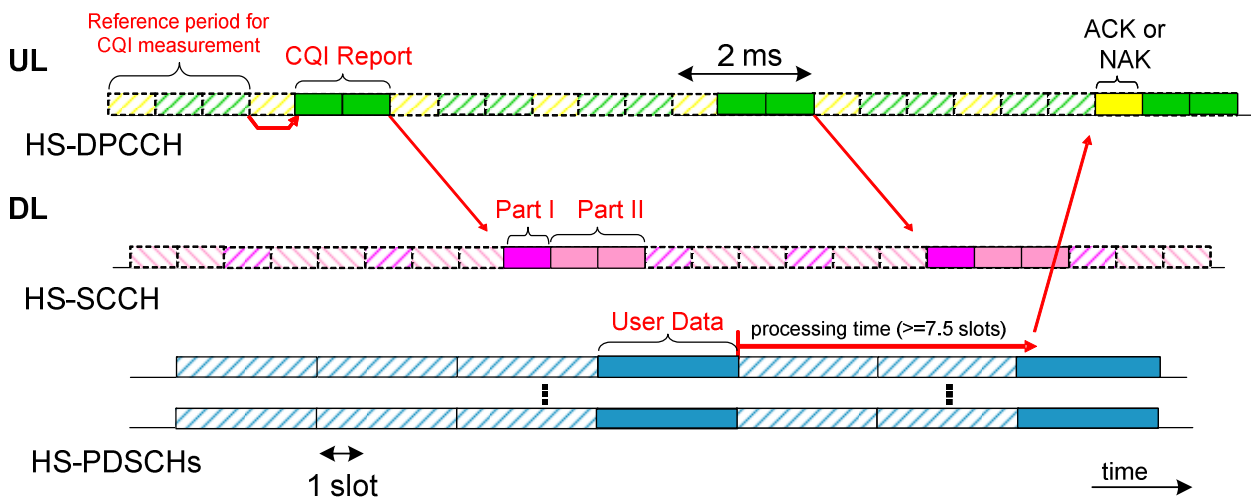
Figure 4.7.2.1-1: Transmission waveform and timing using the existing HS-DSCH subframe format
