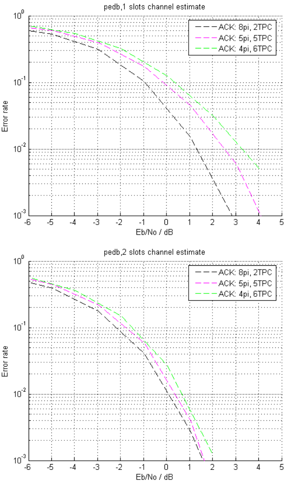
Figure 4.1.2.2-2: ACK performance in PB3, 1 and 2 slot channel estimation, both with TPC-assistance
