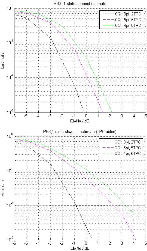
Figure 4.1.2.2.1-3: CQI performance in PB3, 1 slot channel estimation, with and without TPC-assistance
