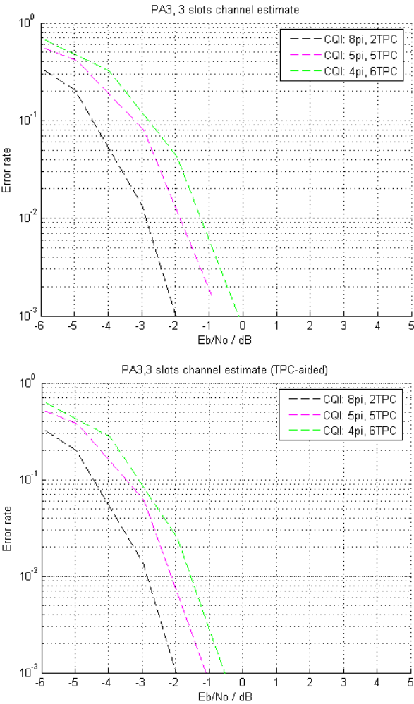
Figure 4.1.2.1-2: CQI performance in PA3, 3 slot channel estimation, with and without TPC-assistance
