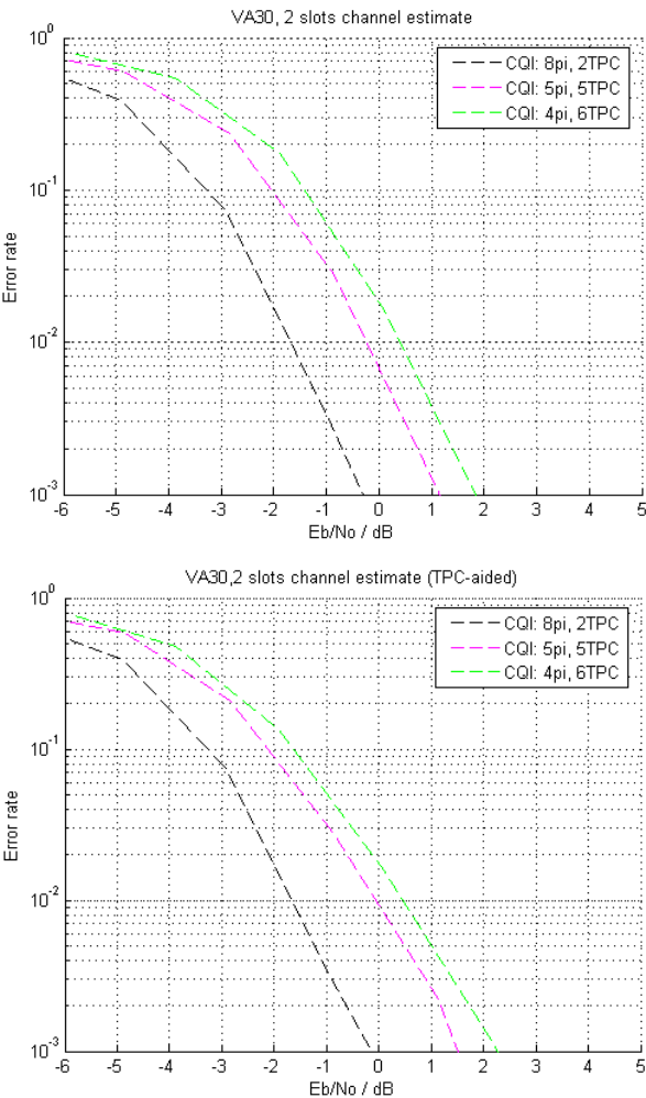
Figure 4.1.2.1-6: CQI performance in VA30, 2 slot channel estimation, with and without TPC-assistance
